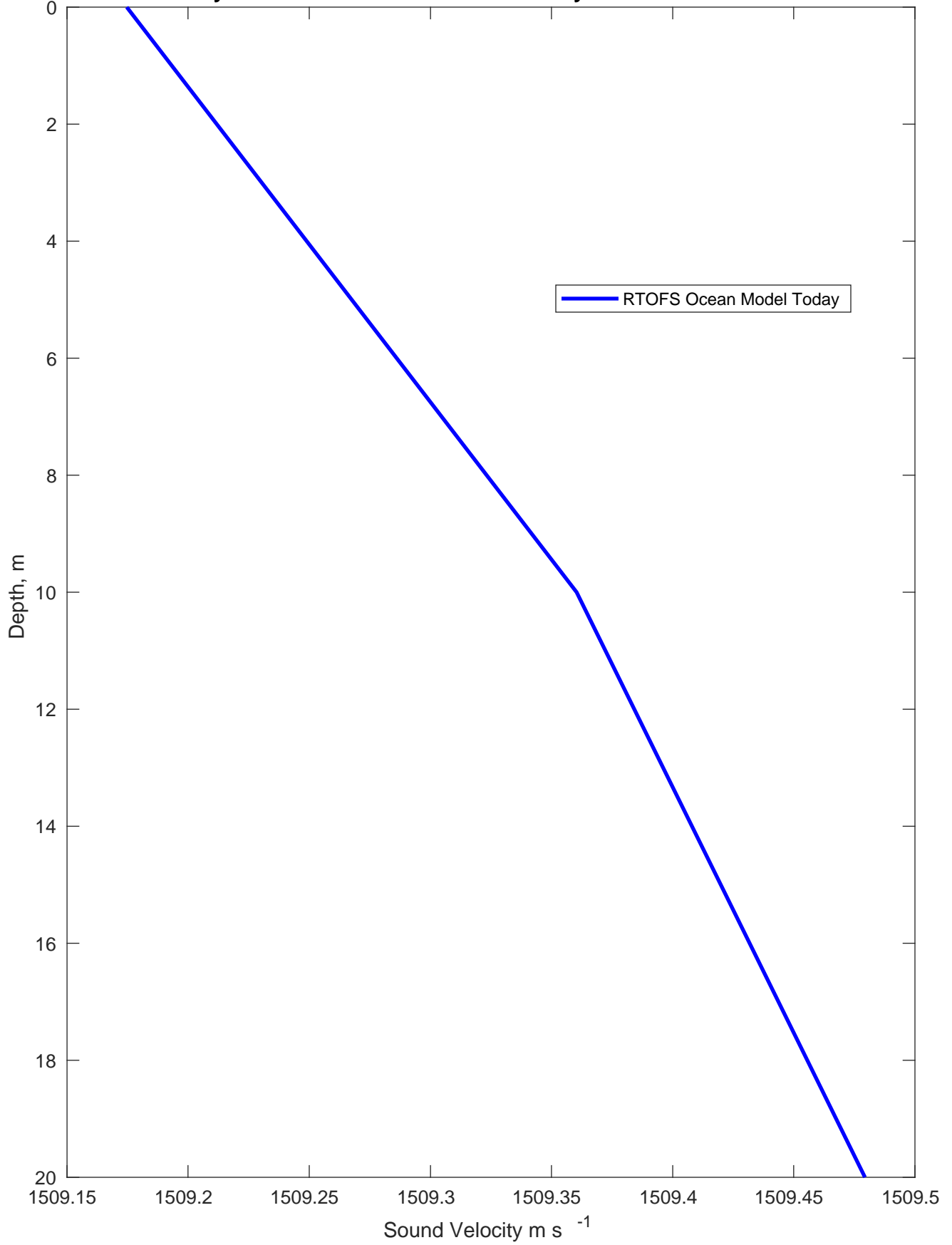
Sound Velocity Profile for US Wind MetOcean Buoy on 08-Nov-2021 00:00:00
